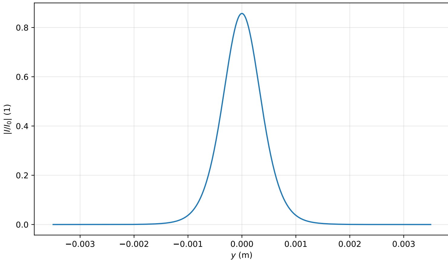
Intensity profile I(x = 0, y, z = 2.309)/I_0 , P_{in}=0.6P_{cr} , artificial time
